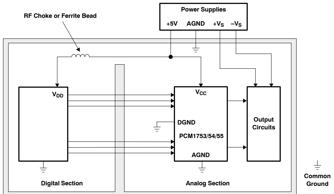
Figure 31. Single-Supply PCB Layout
