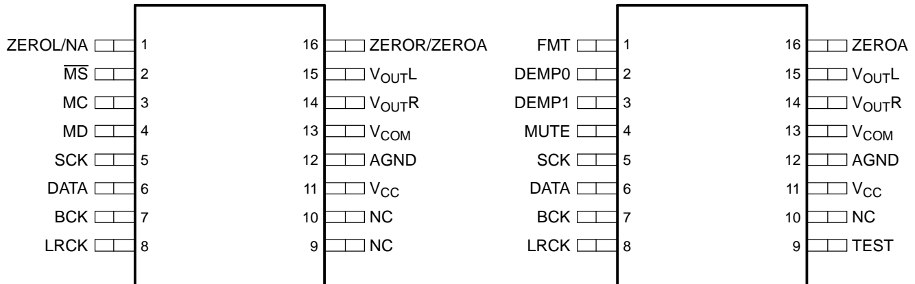
PCM1780/PCM1782 (TOP VIEW)
