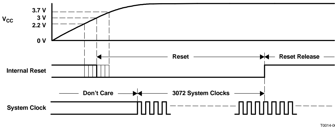
Figure 21. Power-On-Reset Timing
