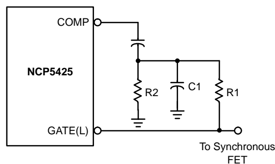
Figure 16. RC Filter Provides the Proper Voltage Ramp at the Beginning of each On-Time Cycle
