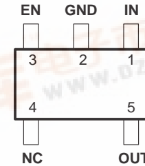
DBV PACKAGE (TOP VIEW)
