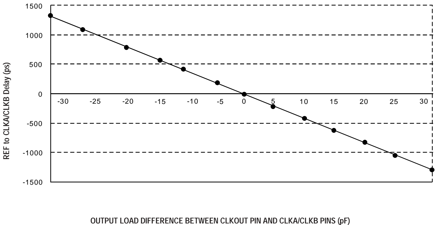
REF TO CLKA/CLKB RELAY vs. OUTPUT LOAD DIFFERENCE BETWEEN CLKOUT PIN AND CLKA/CLKB PINS
