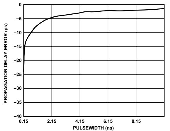
Figure 22. Propagation Delay Error vs. Pulsewidth
