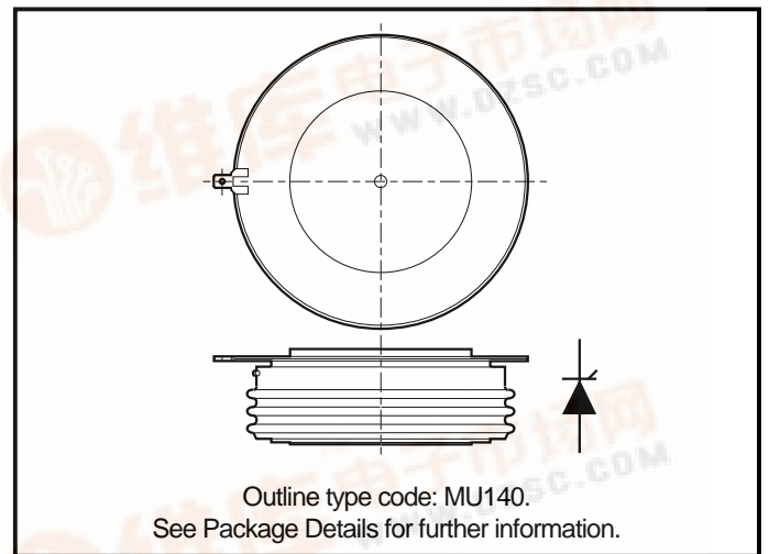
Fig.1 Package outline
