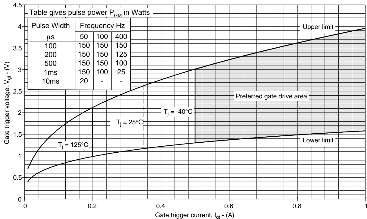
Fig.7 Gate characteristics
