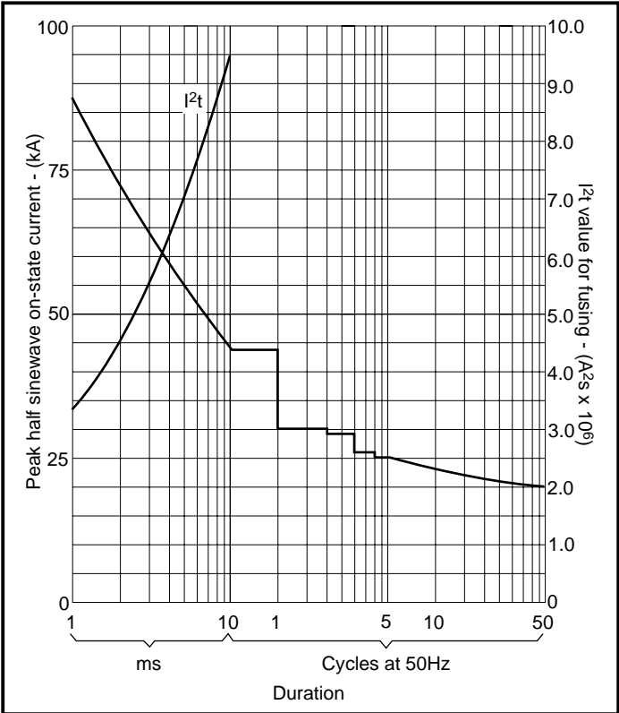
Fig.10 Surge (non-repetitive on-state current vs time
