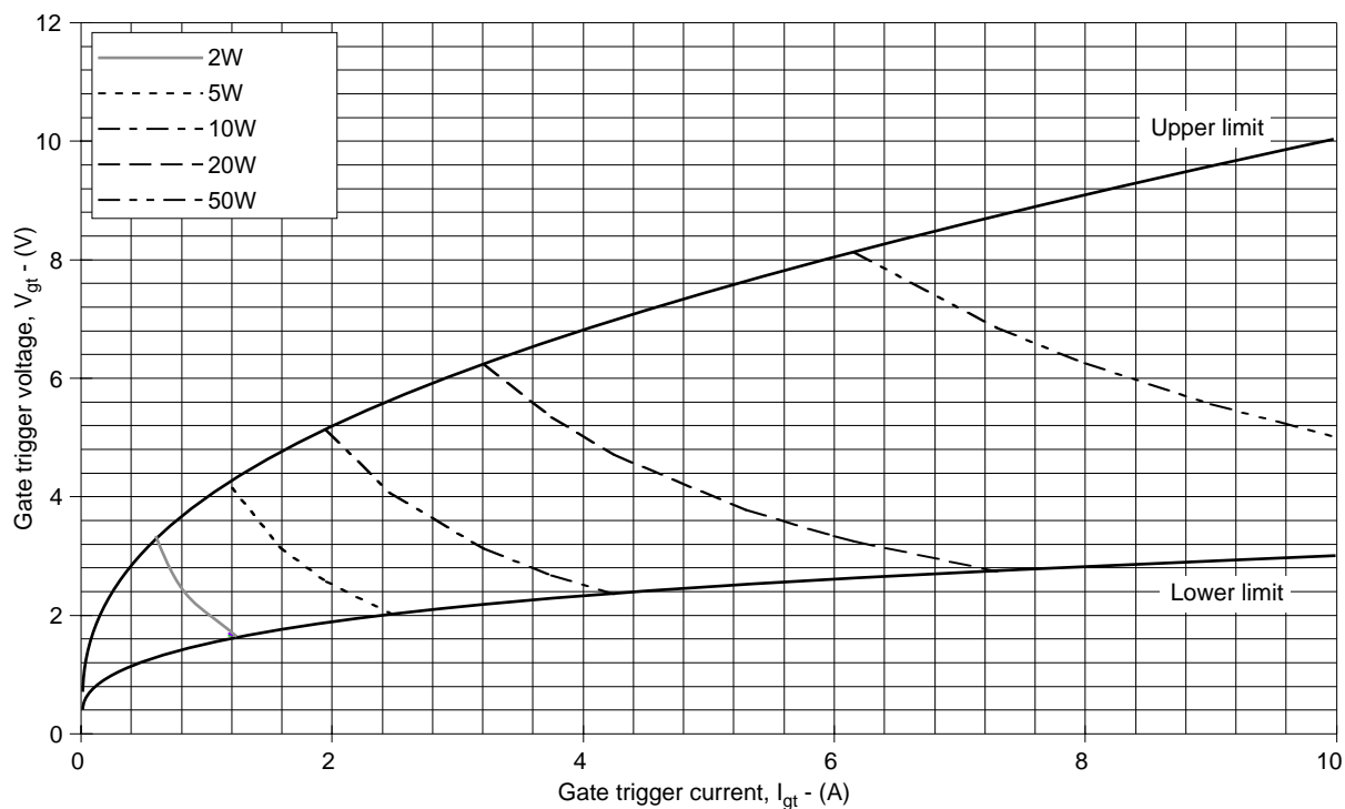
Fig.8 Gate characteristics
