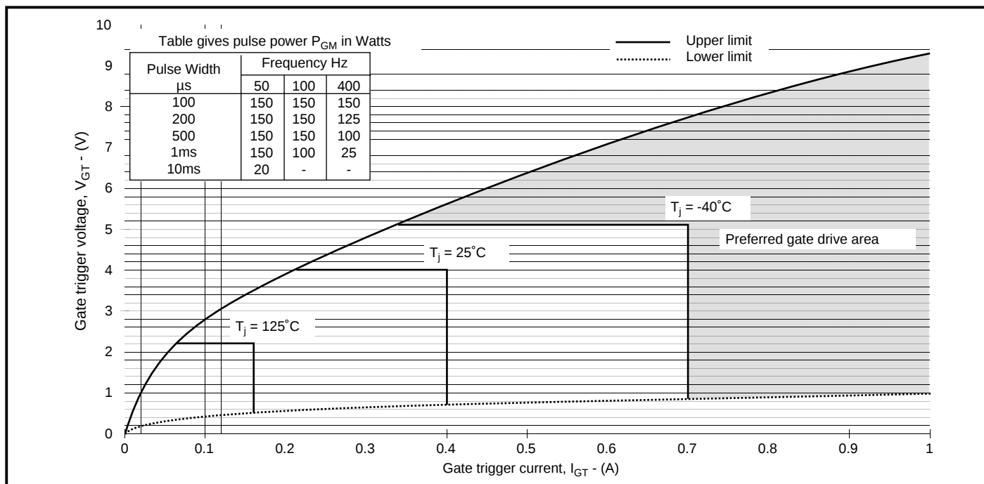
Fig.8 Gate characteristics
