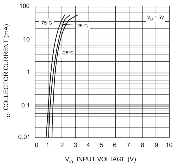
Fig. 10 Collector Current Vs. Input Voltage
