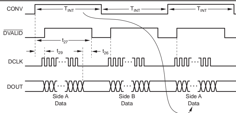
Figure 23. Readback Before CONV Toggles
