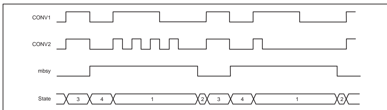
Figure 16. Equivalent CONV Signals in the Non-Continuous Mode
