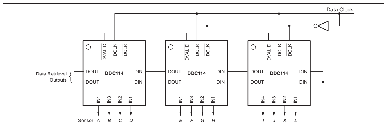
Figure 20. Daisy-Chained DDC114s
