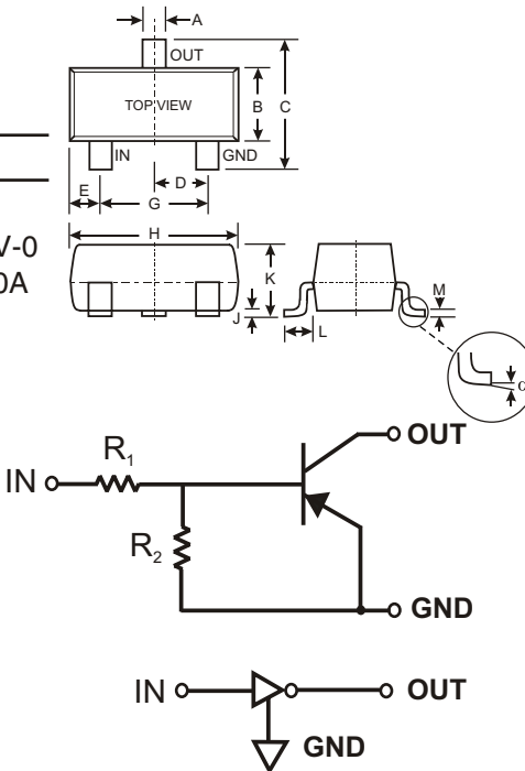
SCHEMATIC DIAGRAM
