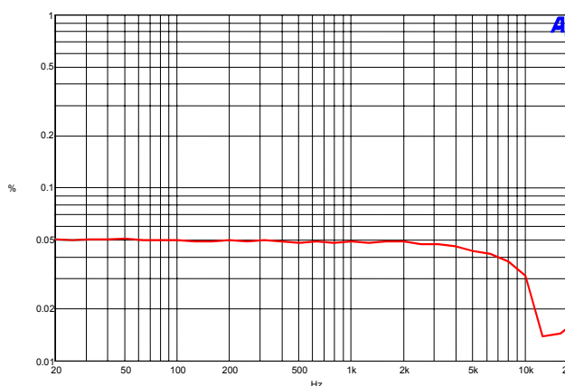
Figure 12. THD+N vs. Frequency, 1W
