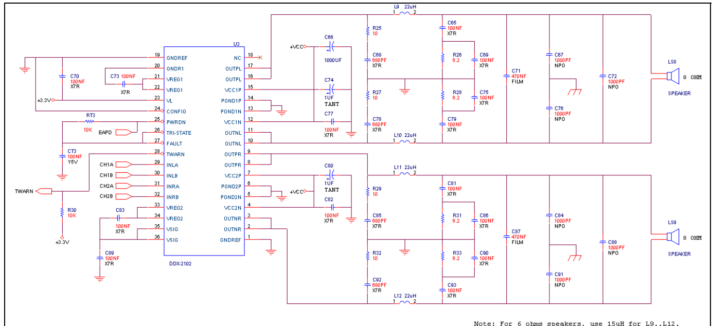
Figure 19. DDX® Stereo Mode Audio Application Circuit
