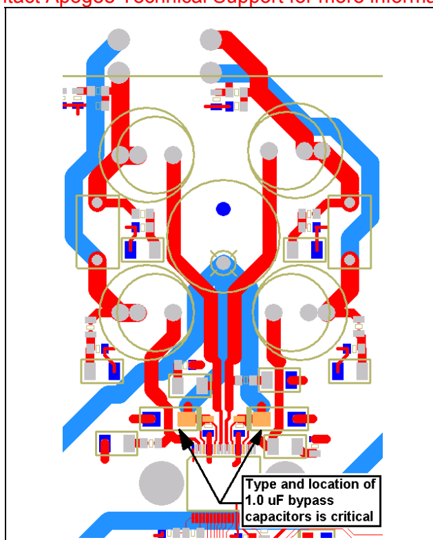
Figure 18 -. Example DDX® Layout (Stereo Mode)
