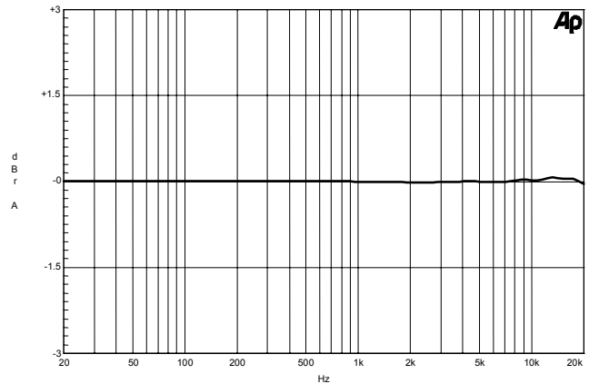
Figure 16. Typical Frequency Response
