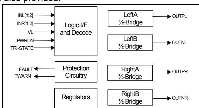
Figure 4 - DDX-2102 Block Diagram, Binary Half-Bridge Mode
