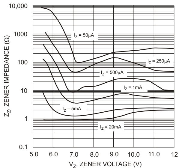
Fig. 10 Typical Zener Impedance Characteristics, DDZX5V6BTS - DDZX12CTS
