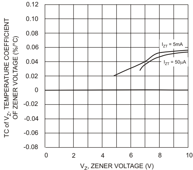
Fig. 16 Typical Temperature Coefficient of Zener Voltage vs. Zener Voltage, DDZX9692 - DDZX9697
