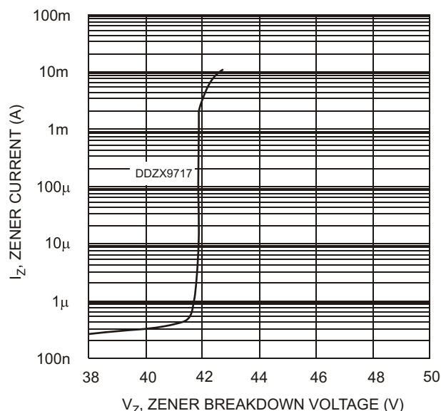
Fig. 9 Typical Reverse Characteristics, DDZX9717
