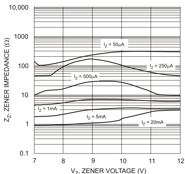
Fig. 11 Typical Zener Impedance Characteristics, DDZX9693 - DDZX9699
