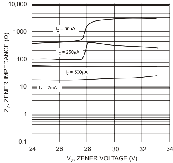
Fig. 14 Typical Zener Impedance Characteristics, DDZX9709 - DDZX9714
