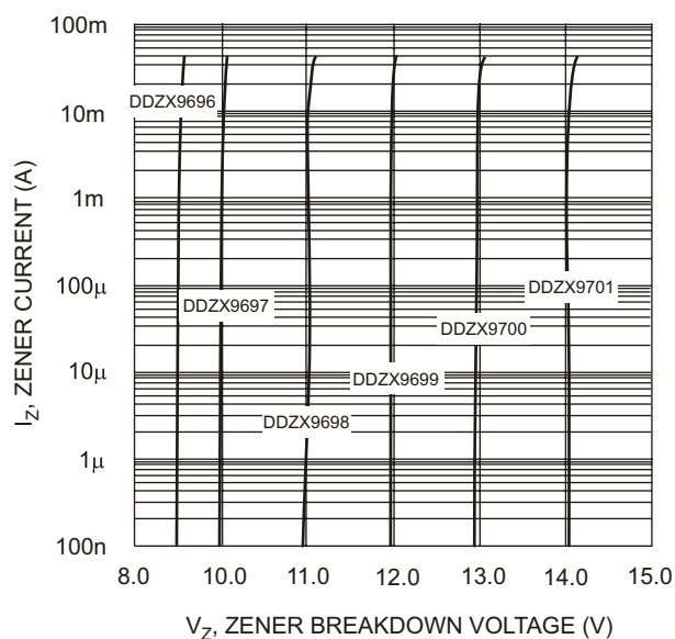
Fig. 5 Typical Reverse Characteristics, DDZX9696 - DDZX9701
