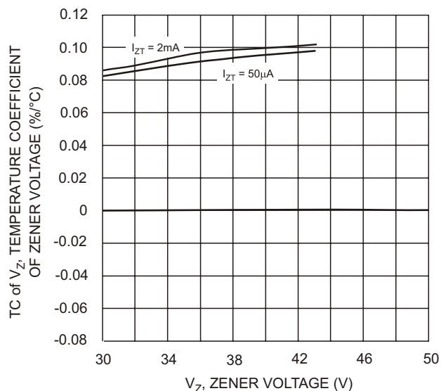
Fig. 19 Typical Temperature Coefficient of Zener Voltage, DDZX9713 - DDZX9717
