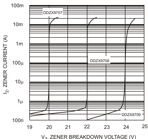
Fig. 7 Typical Reverse Characteristics, DDZX9707 - DDZX9709
