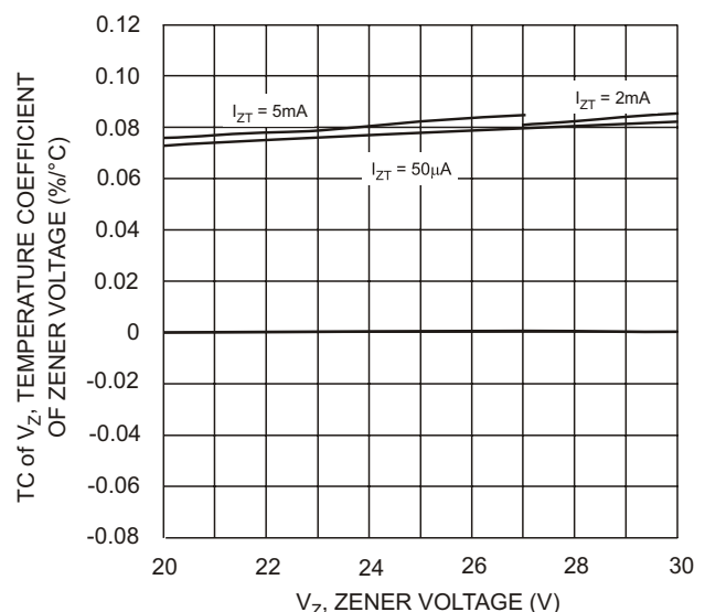
Fig. 17 Typical Temperature Coefficient of Zener Voltage, DDZX20C-DDZX30D
