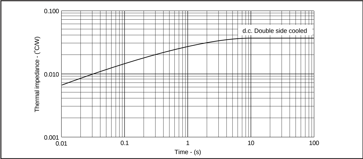
Fig. 6 Maximum (limit) transient thermal impedance - junction to case - ( ^{\circ}\text{C/W} )
