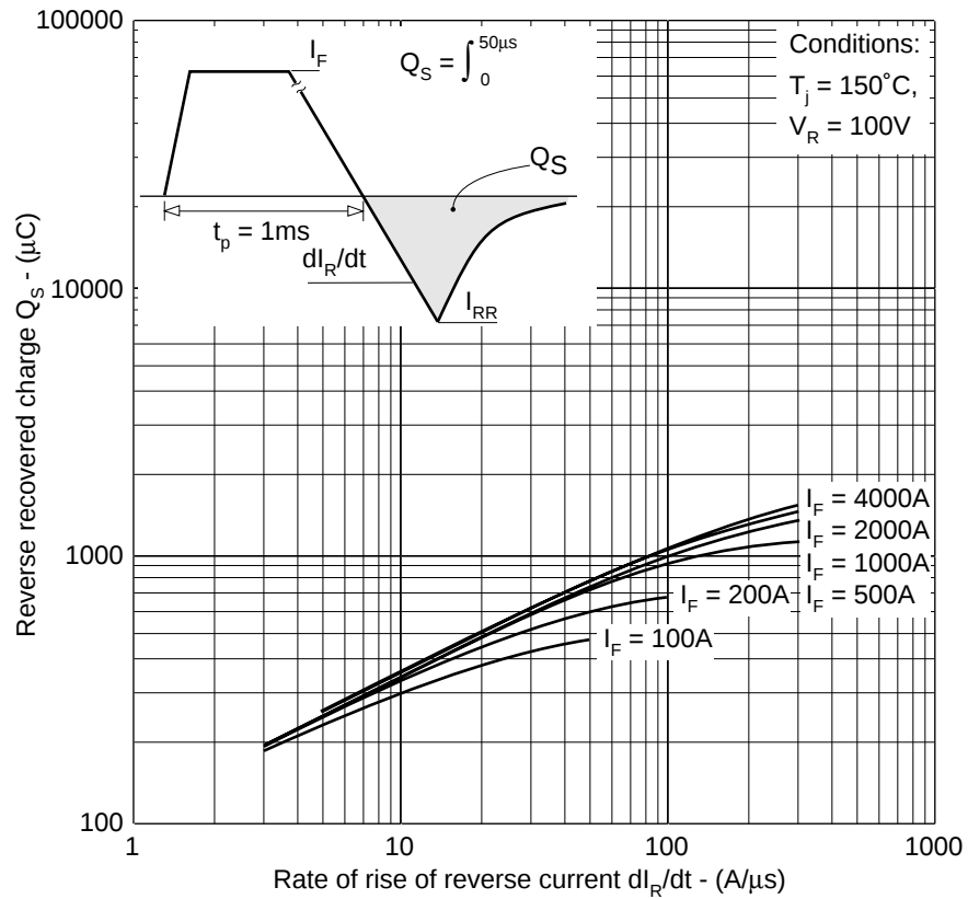
Fig. 4 Recovered charge
