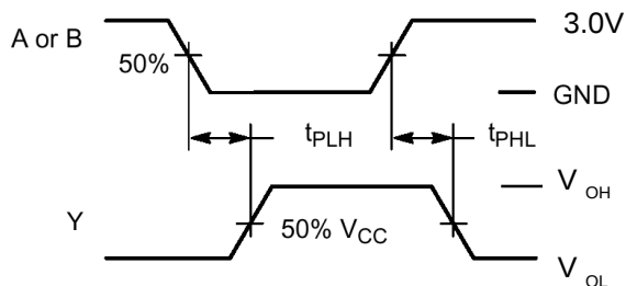
Figure 4. Switching Waveforms
