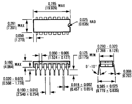
16 Lead Cerdip \theta_{JA} = 100^{\circ}\text{C/W} \theta_{JC} = 60^{\circ}\text{C/W}
