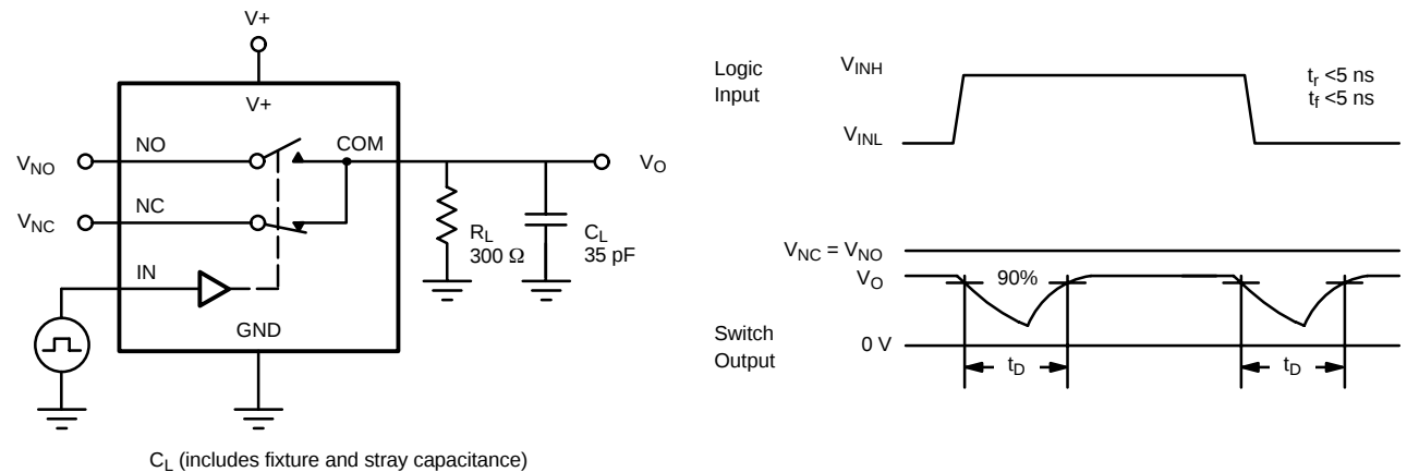
FIGURE 2. Break-Before-Make Interval
