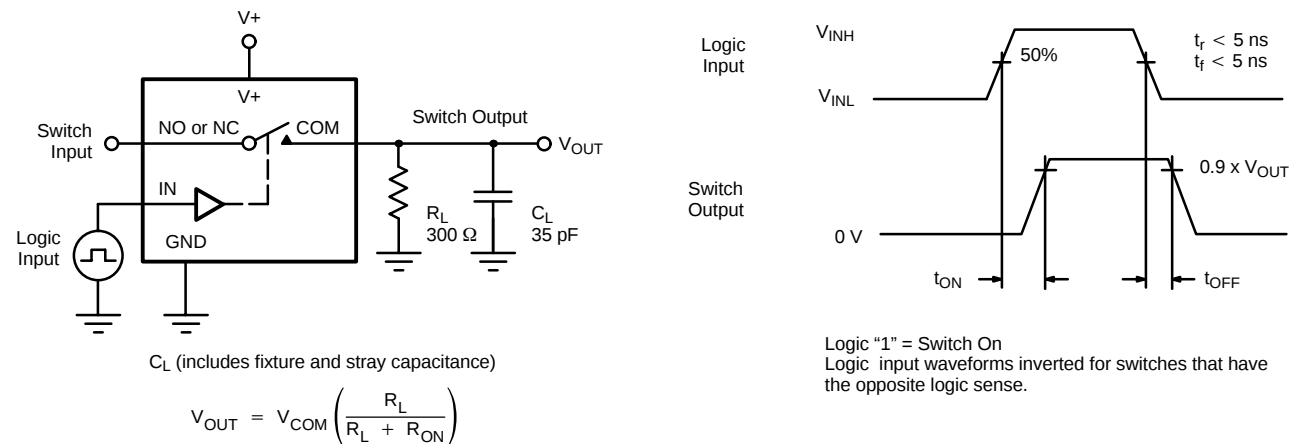
FIGURE 1. Switching Time
