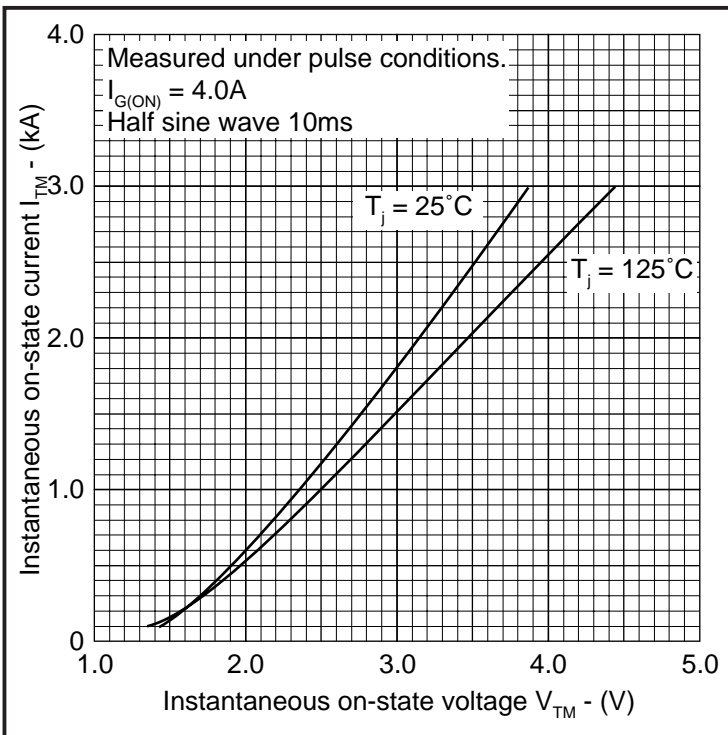
Fig.2 On-state characteristics
