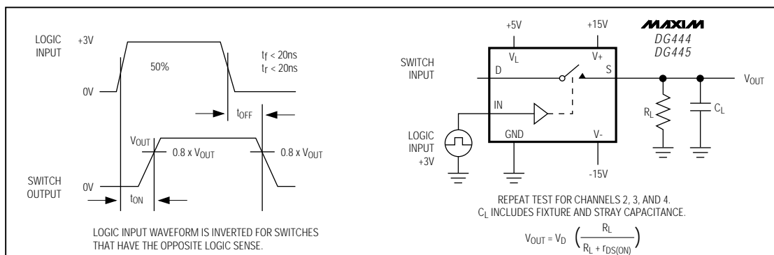
Figure 2. Switching Time
