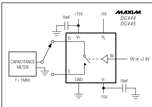
Figure 6. Source/Drain-Off Capacitance
