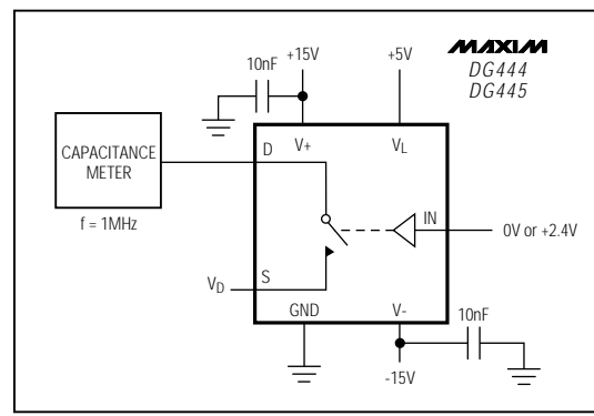
Figure 7. Source/Drain-On Capacitance
