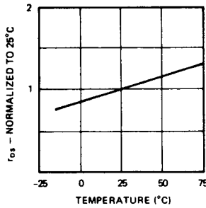
r DS(ON) vs TEMPERATURE (Normalized to 25°C Value)
