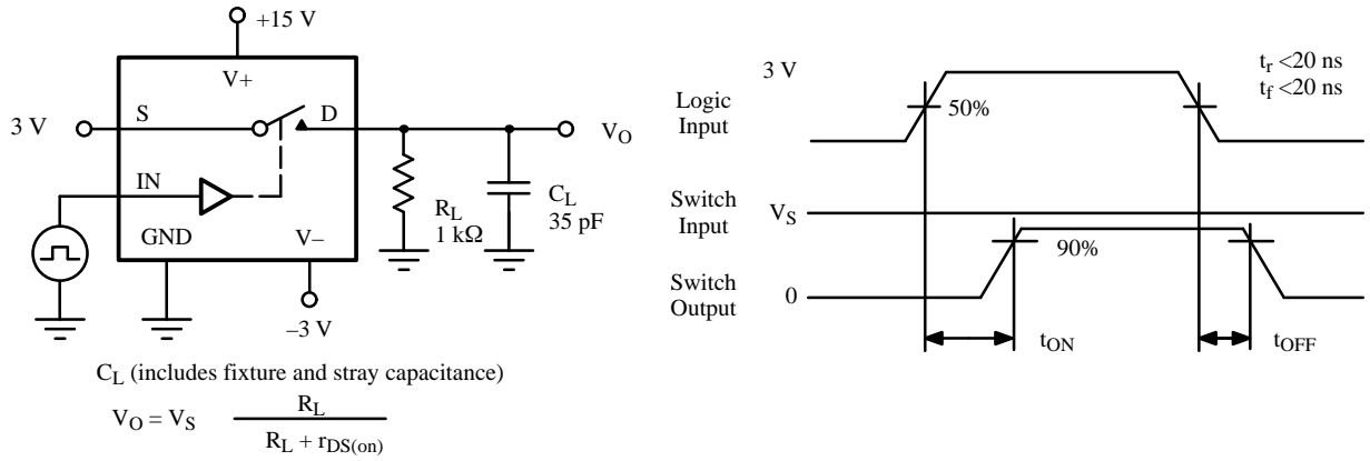
Figure 2. Switching Time
