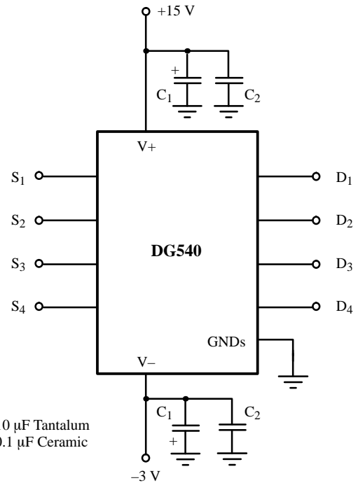
Figure 7. Supply Decoupling
