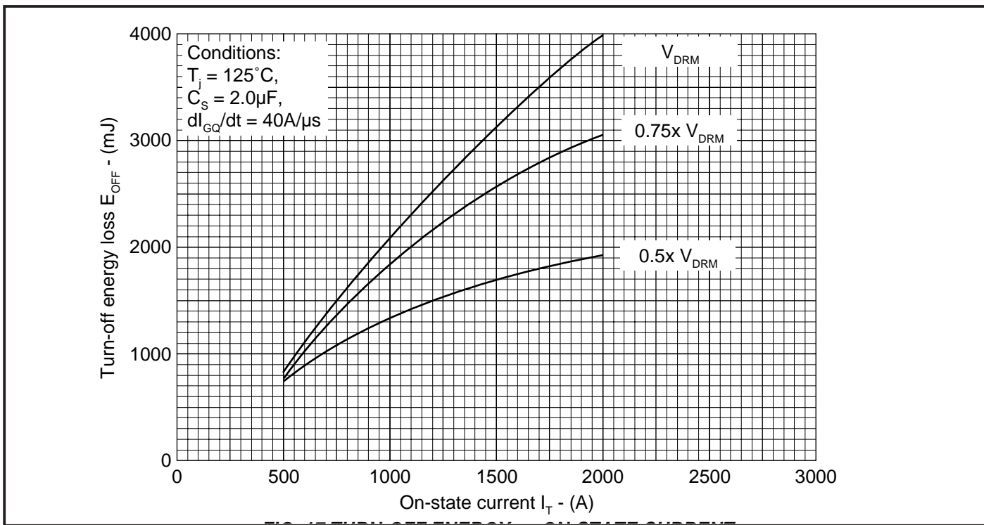
Fig.17 Turn-off energy vs on-state current
