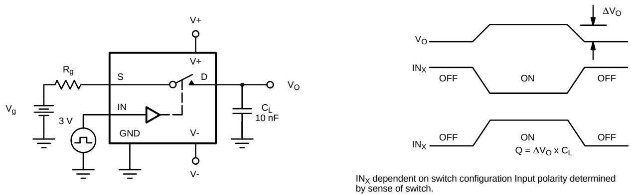
FIGURE 3. Charge Injection
