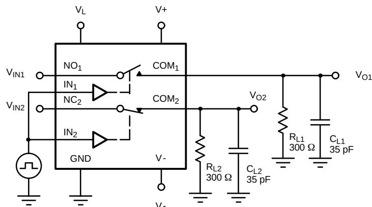
FIGURE 2. Switching Time
