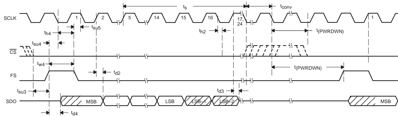
Figure 19. Critical Timing: Control Via CS and FS Inputs (TLC3541 Only)
