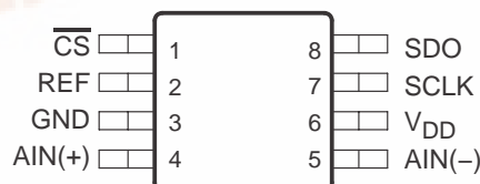
TLC3545 D OR DGK Package (TOP VIEW)
