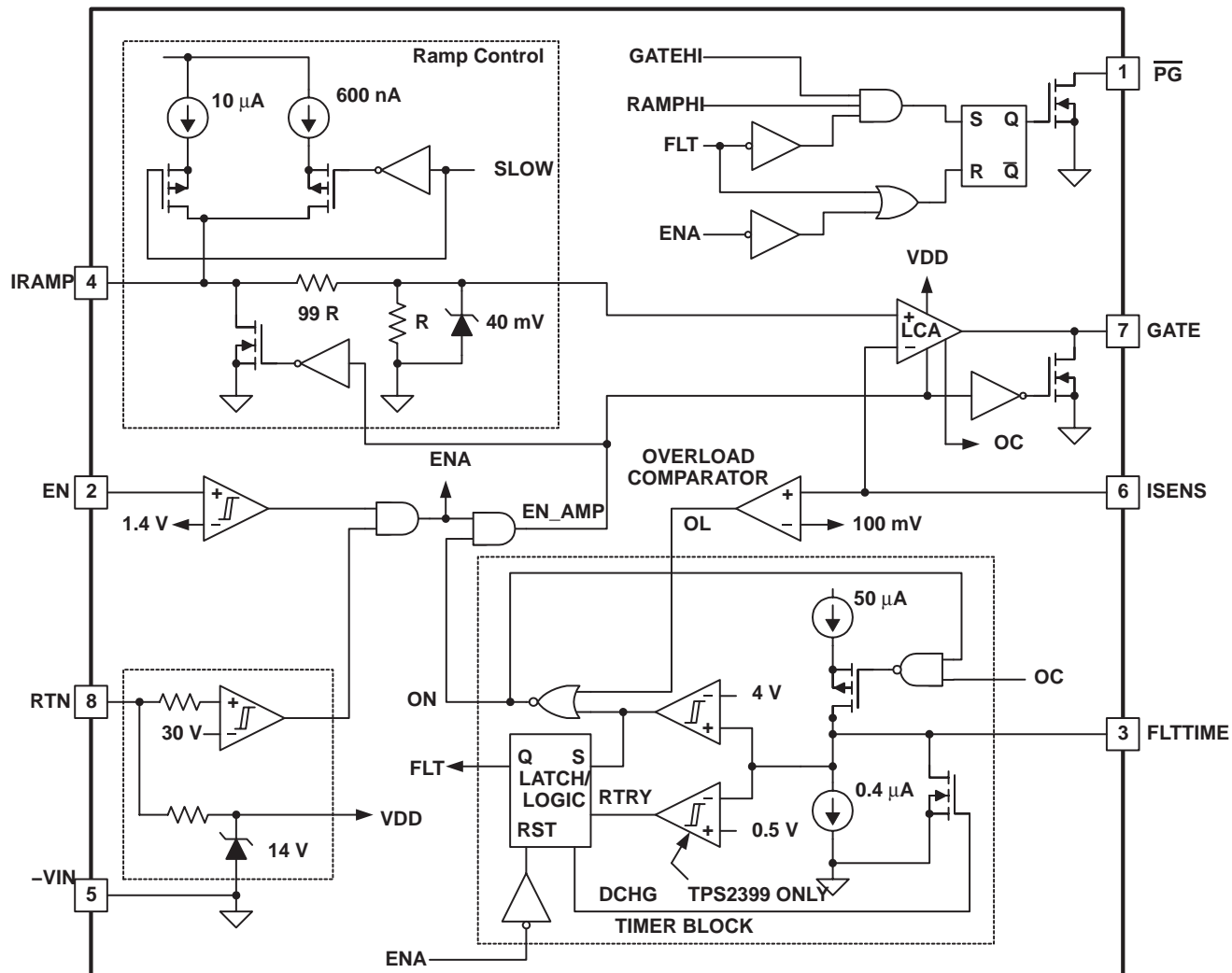
Figure 19. Block Diagram
