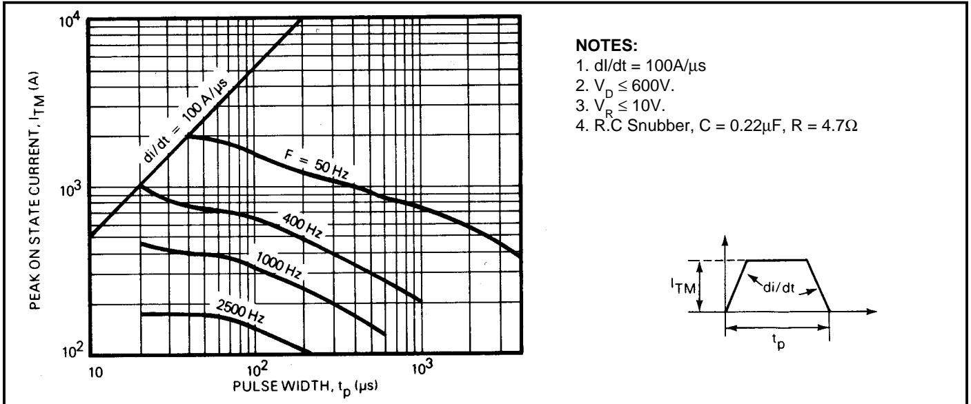
Fig.17 Maximum allowable peak on-state current vs pulse width for T_{\text{case}} = 65^\circ\text{C}
