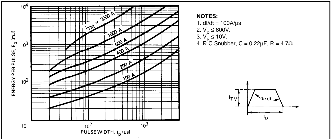
Fig.16 Energy per pulse for trapezoidal pulses
