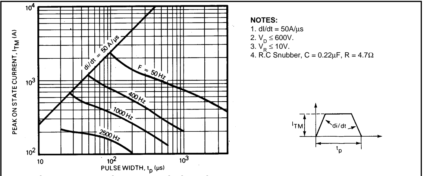
Fig.14 Maximum allowable peak on-state current vs pulse width for T_{case} = 65^\circ C
