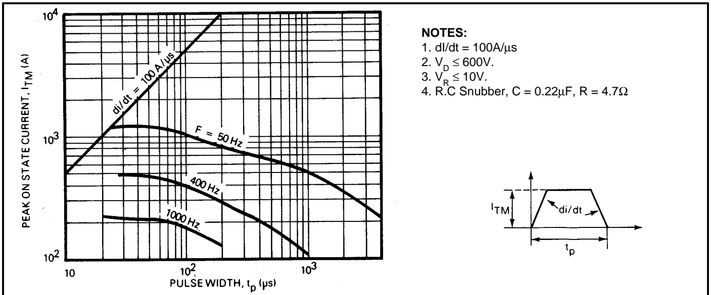
Fig.18 Maximum allowable peak on-state current vs pulse width for T_{\text{case}} = 90^\circ\text{C}
