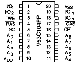
20 Lead Plastic DIP PIN CONFIGURATION Top View
