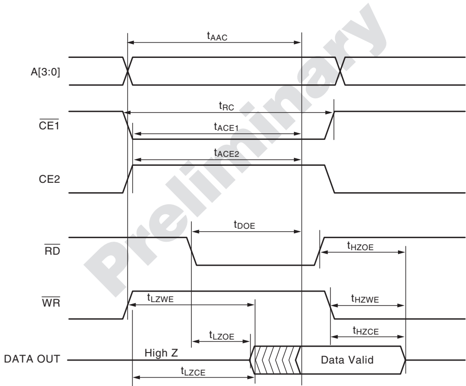
Figure 2. Read Cycle Timing
