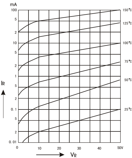
Fig.3 Typical variation of reverse current at various temperatures
