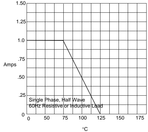
Average Forward Rectified Current - Amperes/ersus Ambient Temperature - °C
