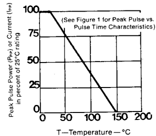
FIGURE 2 DERATING CURVE
