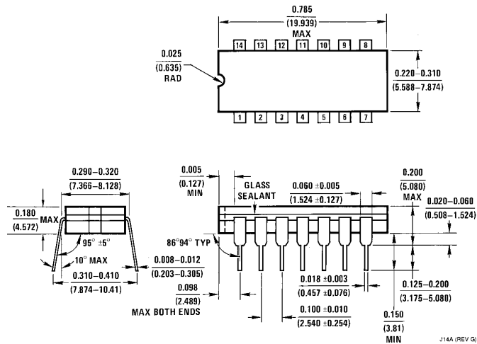
14-Lead Ceramic Dual-In-Line Package (J) Order Number DM5417J NS Package Number J14A
