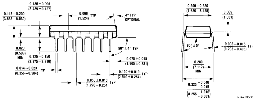
14-Lead Molded Dual-In-Line Package (N) Order Number DM74LS21N NS Package Number N14A
