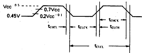
Figure 10. Clock Signal Waveform for I_{CC} Tests in Active and Idle Modes t_{CLH} = t_{CHL} = 5\text{ns}
