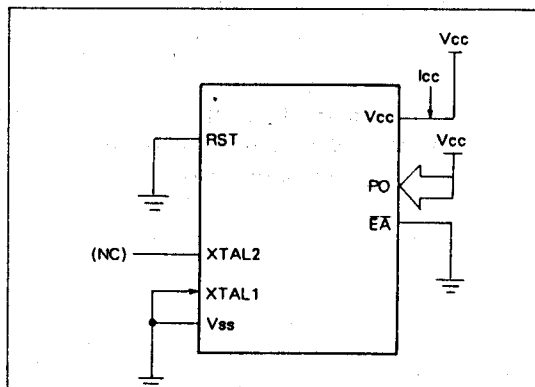
Figure 11. I_{CC} Test Condition, Power down Mode All other pins are disconnected. V_{CC} = 2\text{V to } 5.5\text{V}
