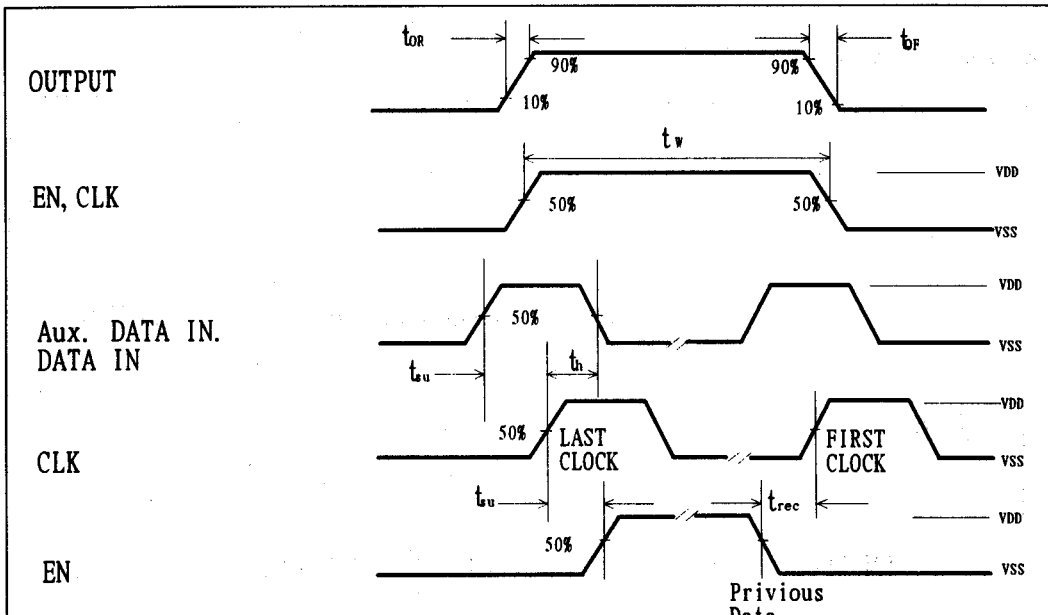
Figure 1. Switching diagram
