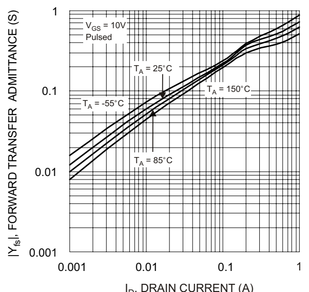
I_D , DRAIN CURRENT (A) Fig. 10 Forward Transfer Admittance vs. Drain Current
