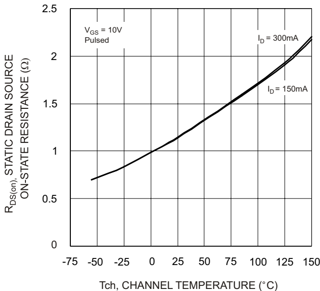
T_{ch} , CHANNEL TEMPERATURE ( ^{\circ}C ) Fig. 7 Static Drain-Source On-State Resistance vs. Channel Temperature
