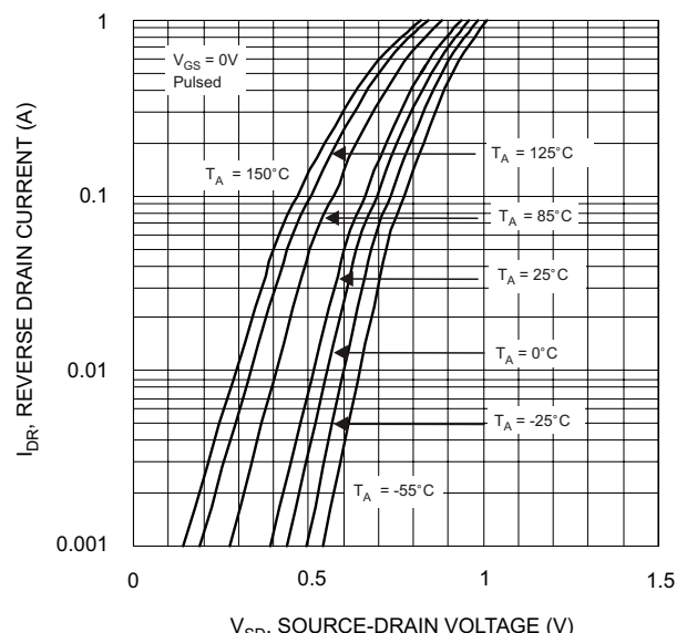
V_{SD} , SOURCE-DRAIN VOLTAGE (V) Fig. 8 Reverse Drain Current vs. Source-Drain Voltage
