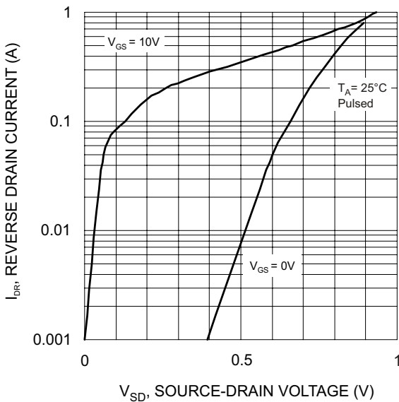
V_{SD} , SOURCE-DRAIN VOLTAGE (V) Fig. 9 Reverse Drain Current vs. Source-Drain Voltage
