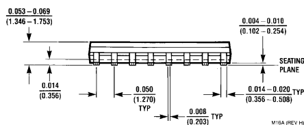
16-Lead Small Outline Molded Package (M) Order Number DM74LS192M NS Package Number M16A
