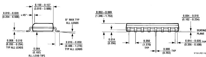
16-Lead Small Outline Molded Package (M) Order Number DM74LS352M NS Package Number M16A
