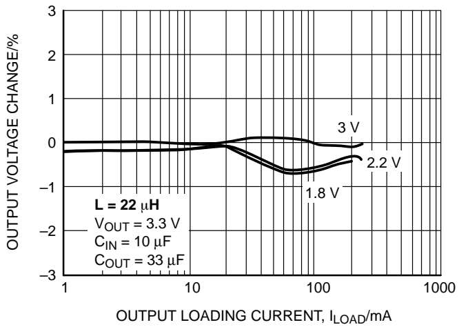
Figure 15. Output Voltage Change versus Load Current
