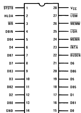
Dual-In-Line Package
