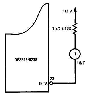
FIGURE 3. INTA Test Circuit (For RST 7)
