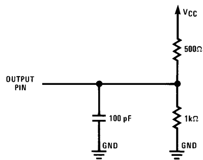
FIGURE 2. Test Load
