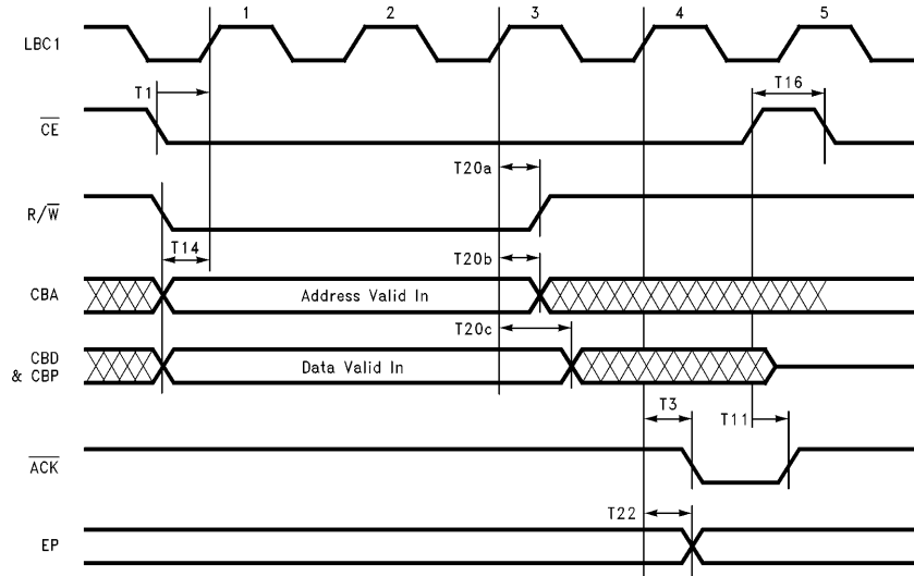
FIGURE 7-3. Control Bus Synchronous Writes
