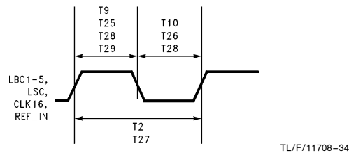
FIGURE 7-8. Clock Pulse Widths
