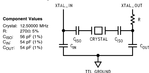
FIGURE 3-19. Crystal Circuit
