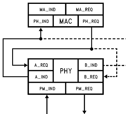
FIGURE 3-11. Single Attachment Station (SAS) Using the DP83257
