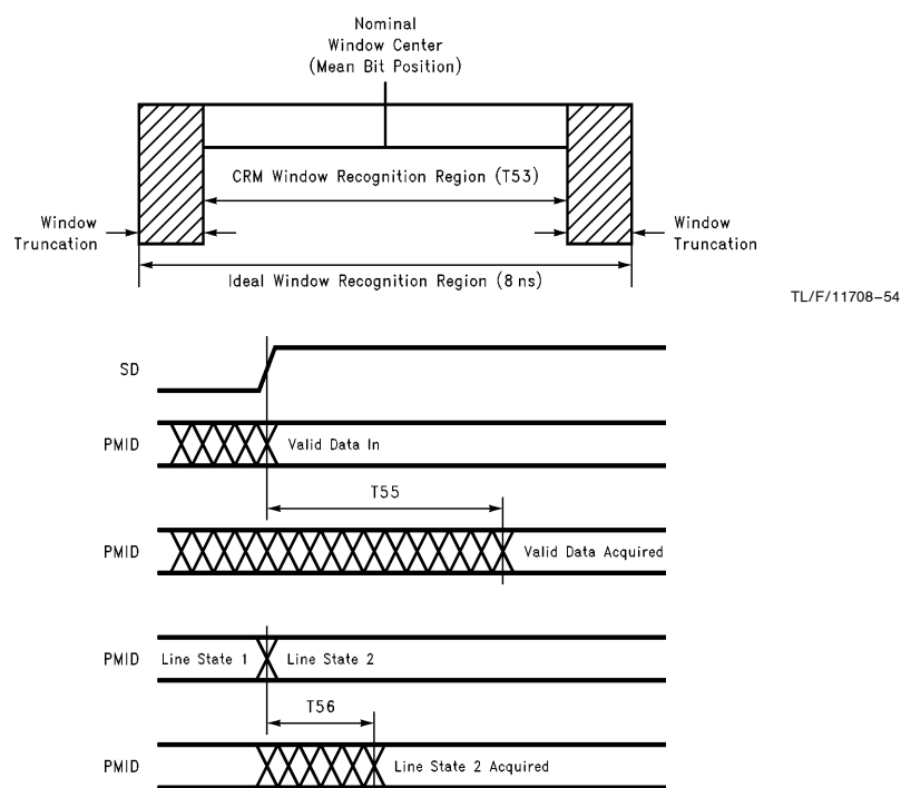
FIGURE 7-13. Alternate PMD Input Timing Diagrams—ANSI Specifications
