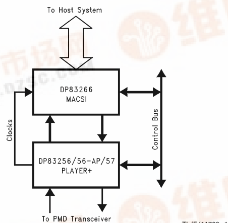
FIGURE 1-1. FDDI Chip Set Overview
