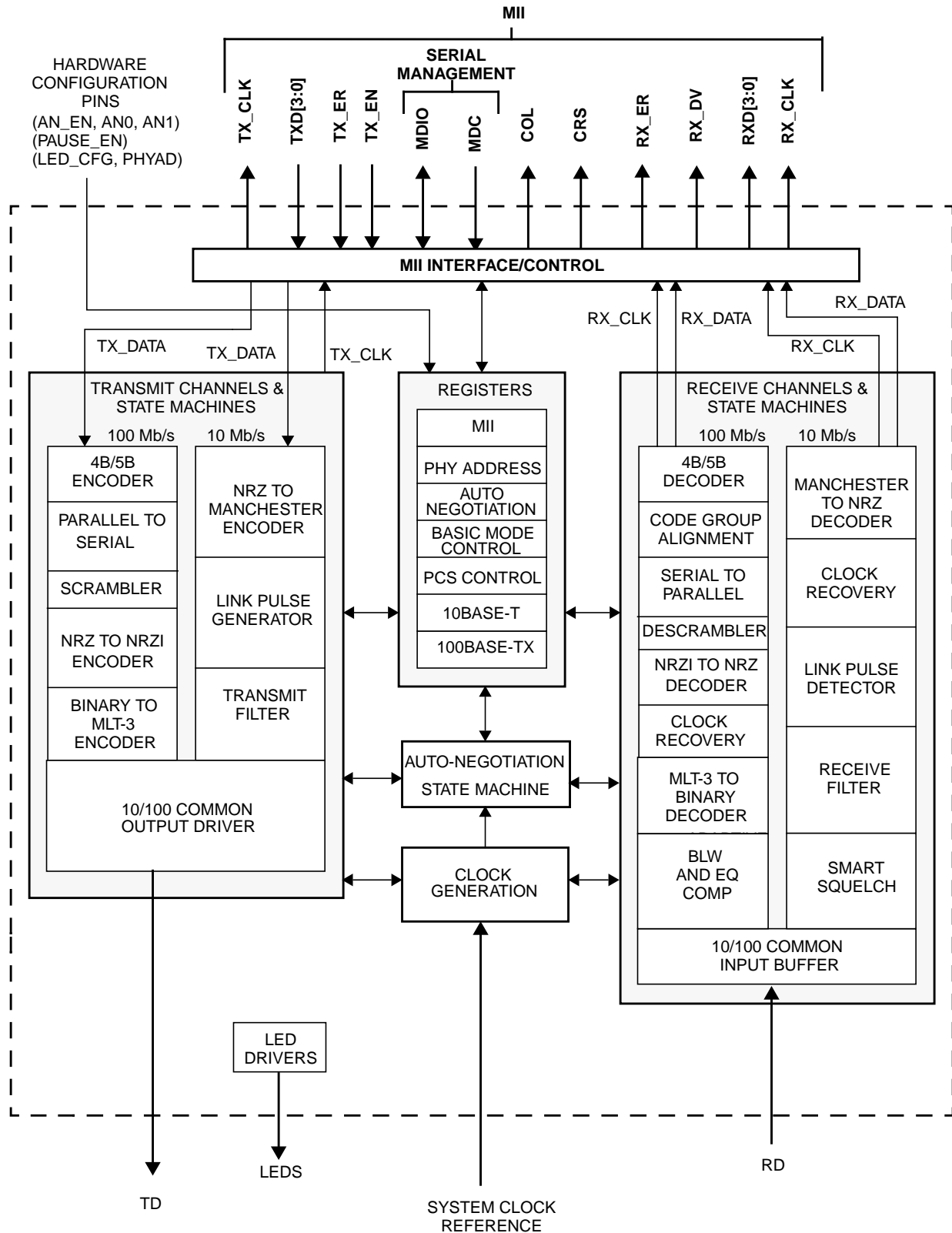
Figure 1. Block Diagram of the 10/100 DSP based core.
