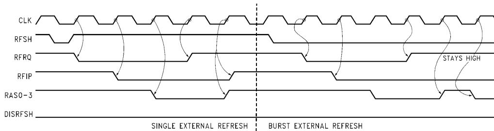
FIGURE 15a. Externally Controlled Single and Burst Refresh with Refresh Request ( \overline{\text{RFRQ}} ) Output (2 Periods of \overline{\text{RAS}} Low during Refresh Programmed)
