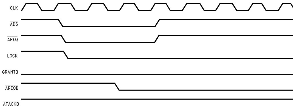
FIGURE 35. \overline{\text{LOCK}} Function
