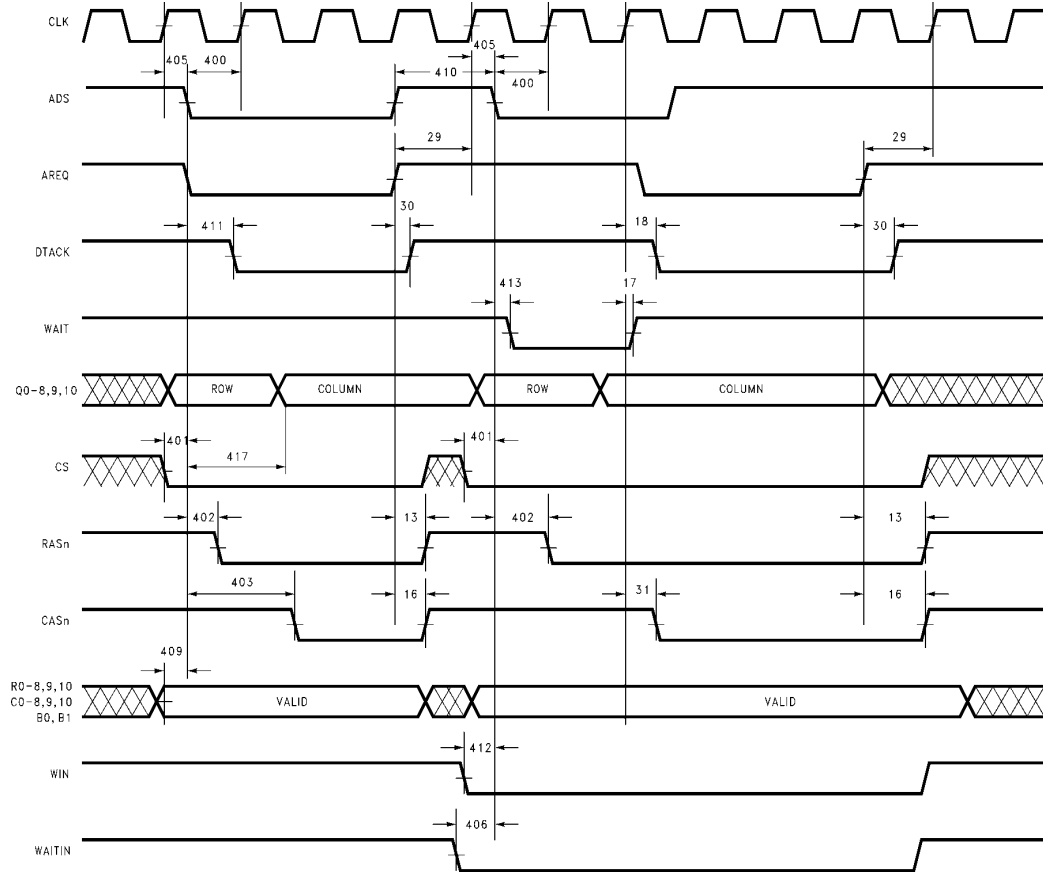
FIGURE 42. 400: Mode 1 Timing
