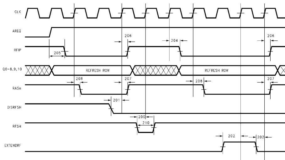
FIGURE 39. 200: Refresh Timing
