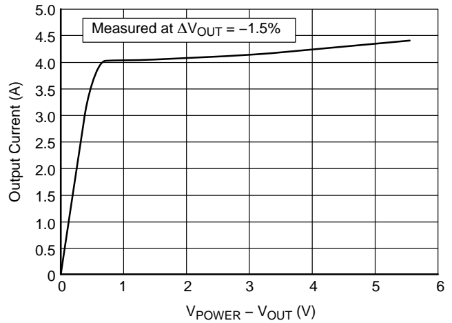
Figure 4. Output Current vs V_{\text{POWER}} - V_{\text{OUT}}
