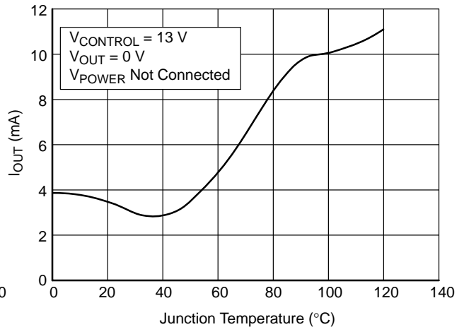
Figure 8. V_{\text{CONTROL}} Only Output Current vs Junction Temperature
