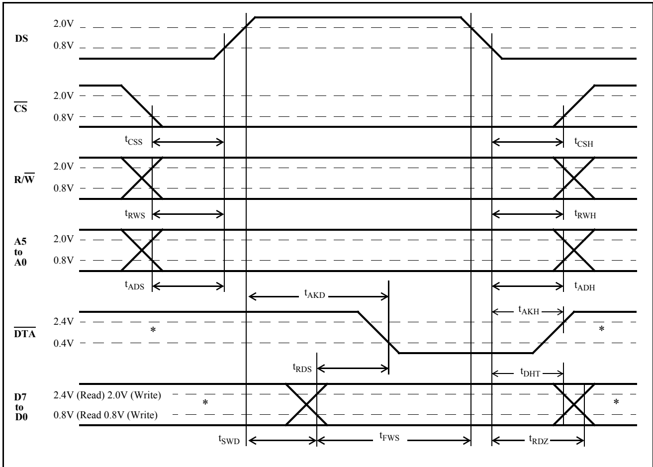
Figure 17 - Processor Bus
