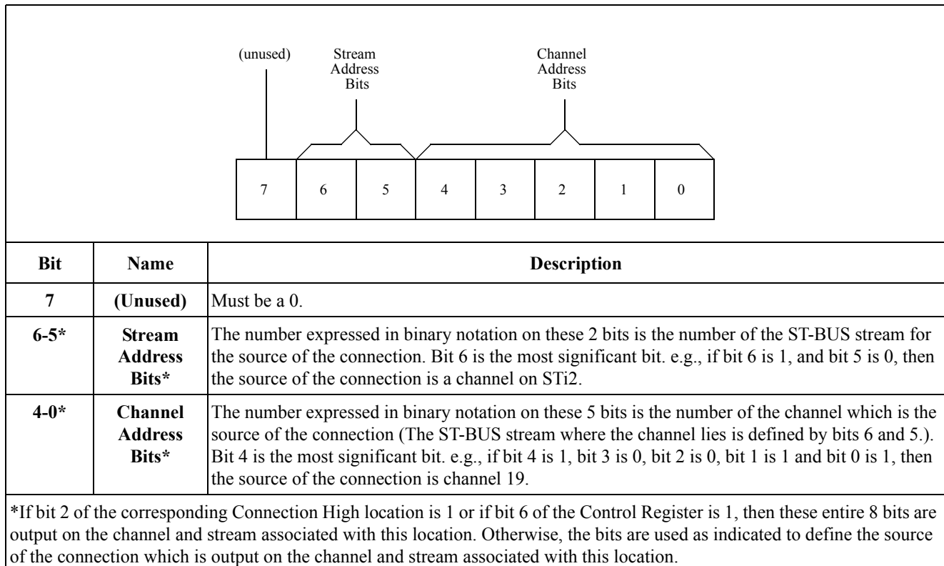
Figure 6 - Connection Memory Low Bits
