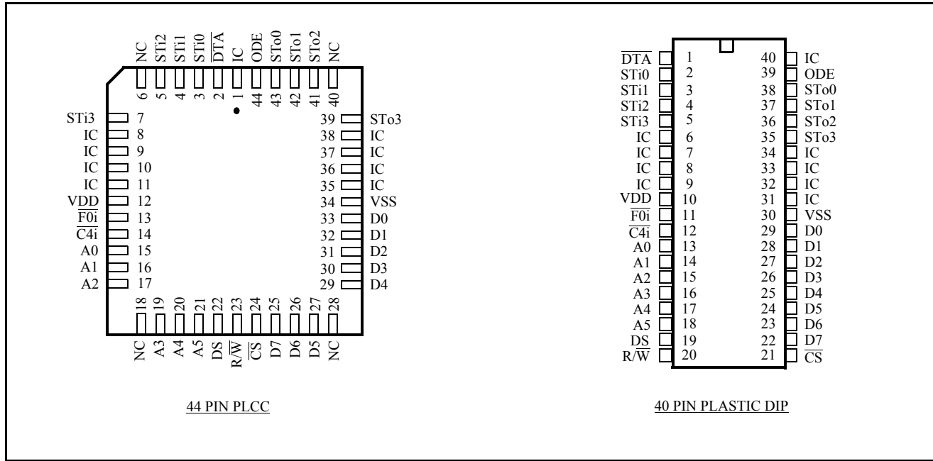
Figure 2 - Pin Connections
