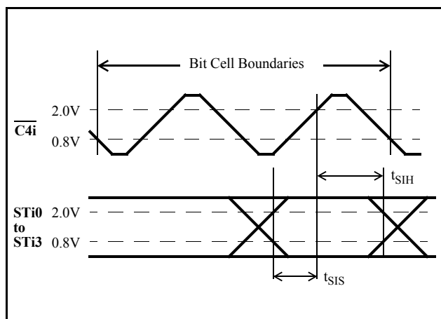
Figure 16 - Serial Inputs
