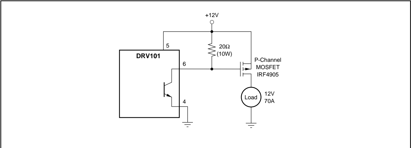
FIGURE 21. High Power, High-Side Driver.
